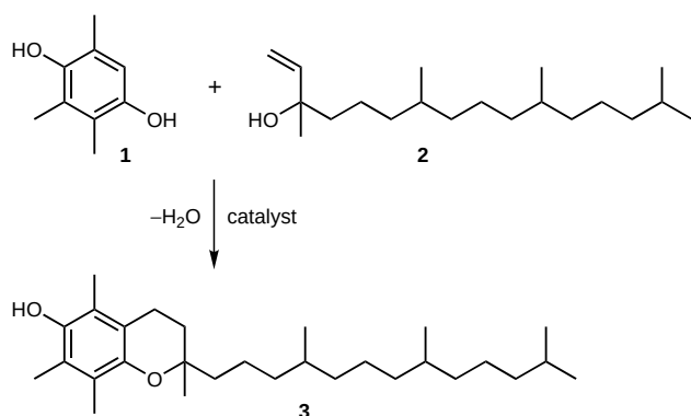
Scheme 1. Synthesis of (all- rac )- \alpha -tocopherol ( 3 ).
