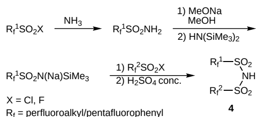
Scheme 2. Preparation of catalysts 4 .
